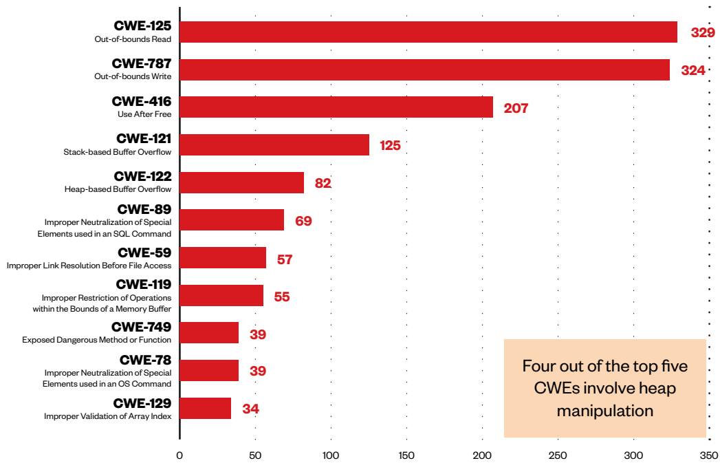
Figure 4. Top 10 CWEs from 2022 Published Advisories
