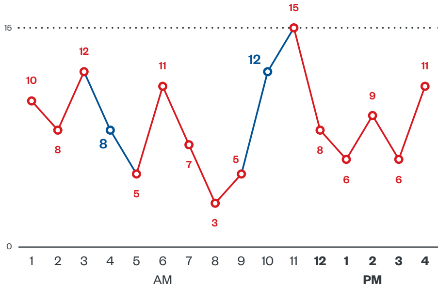
Figure 8. A typical day showing the back-and-forth control of a cloud instance by Kinsing (red) and 8220 (blue), with the numbers representing inbound control connections
